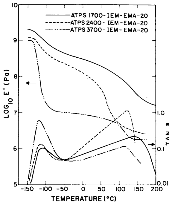
Fig. 8. Effect of ATPS molecular weight on the storage modulus ( E' ) and loss tangent of the ATPS-IEM-EMA-20 materials.
