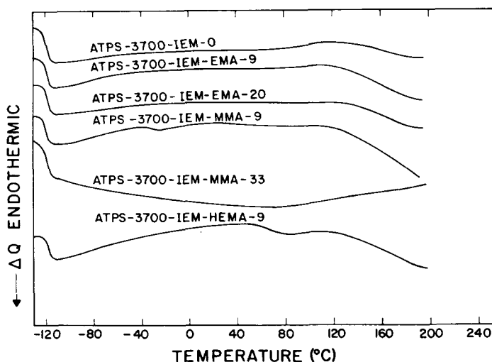
Fig. 4. DSC curves of ATPS-3700-IEM series materials.
