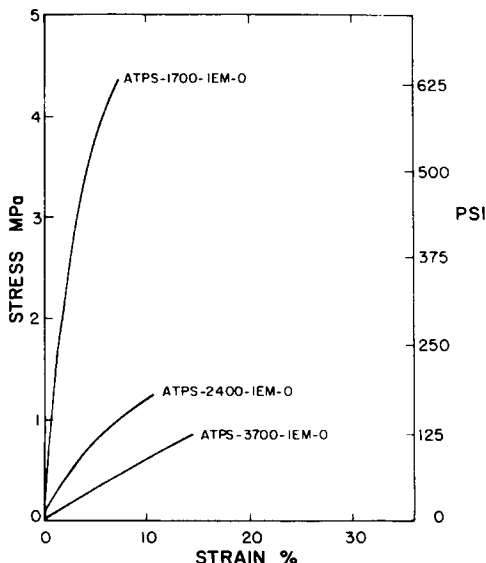
Fig. 5. Effect of ATPS molecular weight on the tensile properties of the ATPS-IEM-0 materials.
