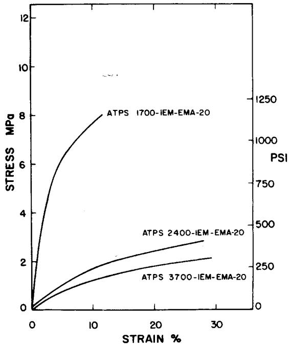
Fig. 7. Effect of ATPS molecular weight on the tensile properties of the ATPS-IEM-EMA-20 system.
