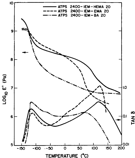
Fig. 14. The storage modulus ( E' ) and loss tangent of ATPS-2400-IEM-20 series materials.
