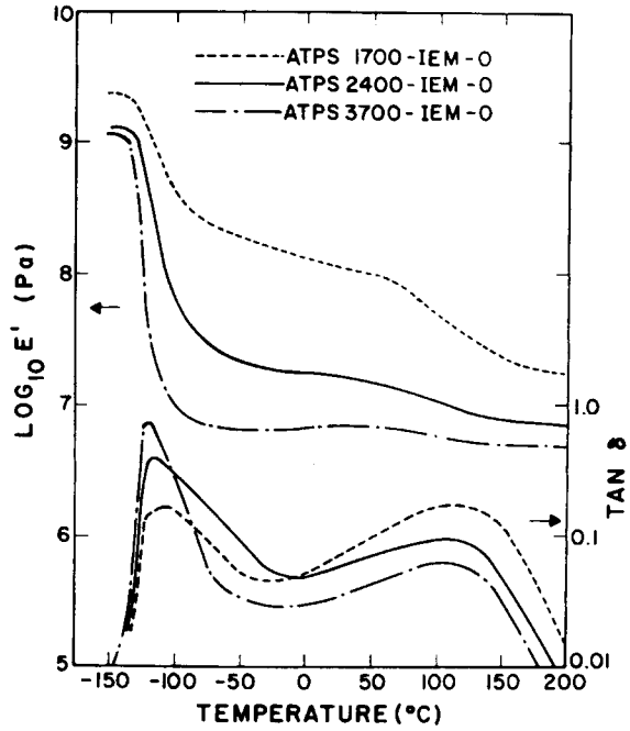
Fig. 6. Effect of ATPS molecular weight on the storage modulus ( E' ) and loss tangent of the ATPS-IEM-0 materials.
