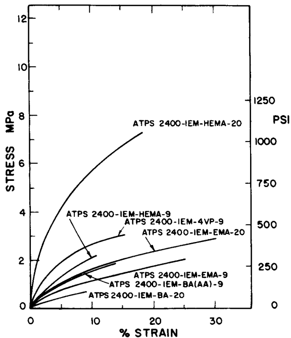
Fig. 13. Effect of HEMA, EMA, BA, 4VP, and BA-AA content on the tensile properties of ATPS-2400-IEM.
