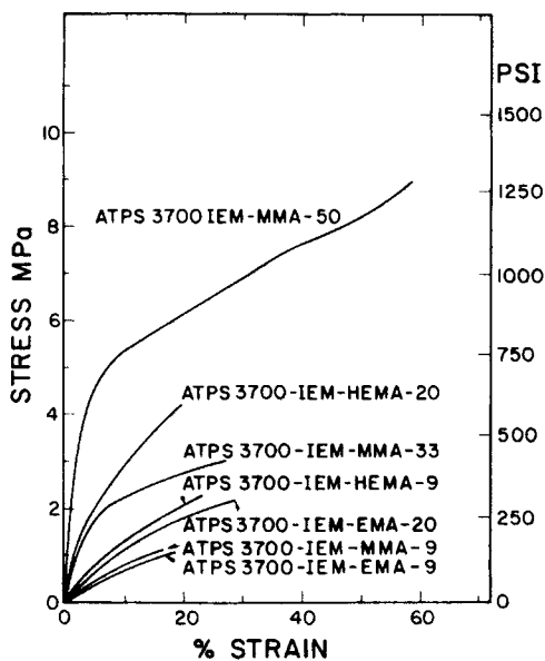
Fig. 10. Effect of MMA, EMA, and HEMA content on the tensile properties of ATPS-3700-IEM.
