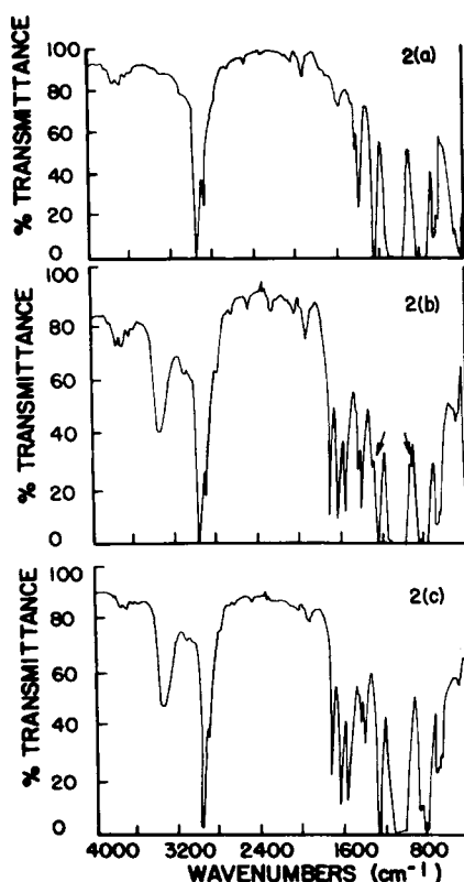
Fig. 2. Infrared spectra of (a) ATPS-2400 oligomer, (b) ATPS-2400-IEM-0 before UV curing, and (c) ATPS-2400-IEM-0 after UV curing.
