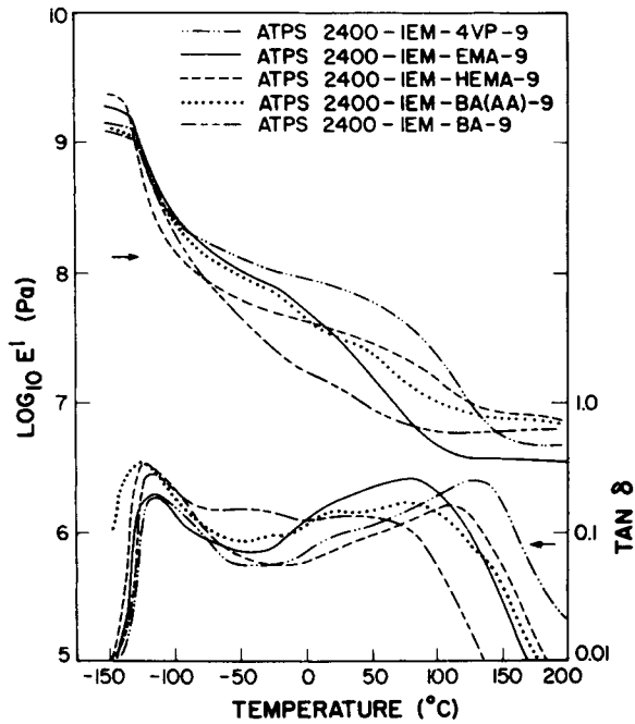
Fig. 12. The storage modulus ( E' ) and loss tangent of ATPS-2400-IEM-9 series materials.
