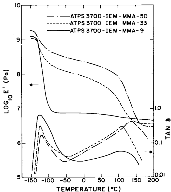
Fig. 9. Effect of MMA content on the dynamic mechanical properties of ATPS-3700-IEM.
