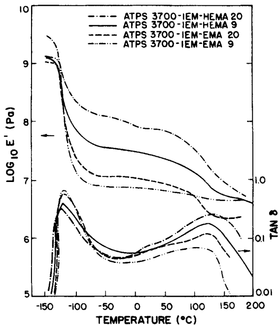
Fig. 11. Effect of HEMA and EMA content on the storage modulus ( E' ) and loss tangent of ATPS-3700-IEM.
