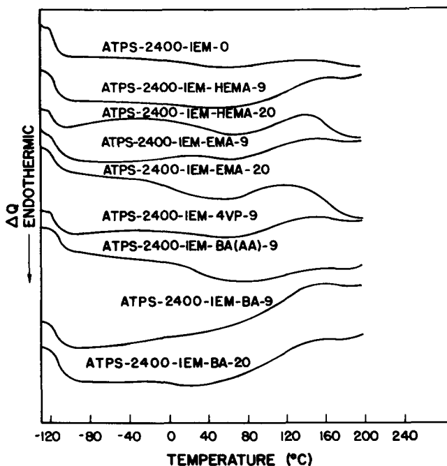
Fig. 3. DSC curves of ATPS-2400-IEM-9 and ATPS-2400-IEM-20 series materials.
